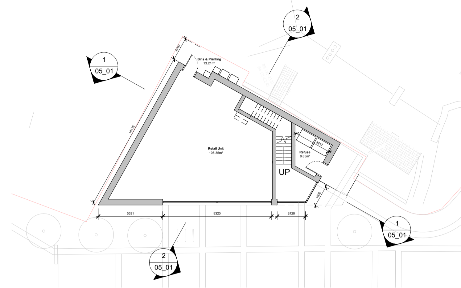
1 Ground Floor Plan 1 : 200
